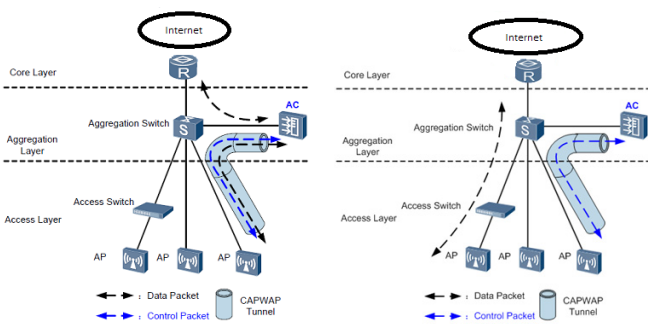
Figure 11: Centralized Switching and Distributed Switching
