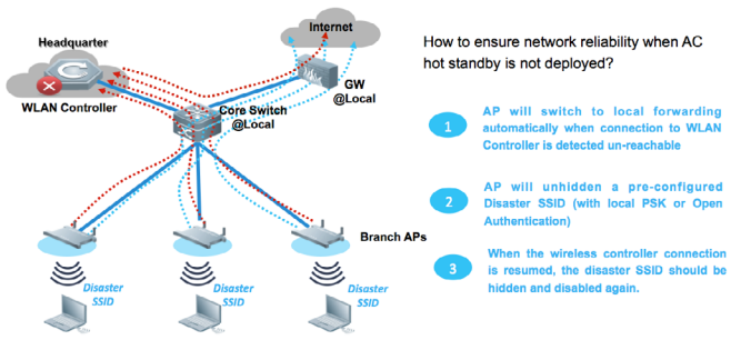
Figure 10: RIPT Disaster Recovery
